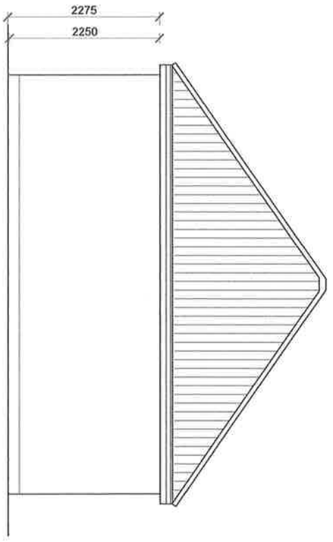
REAR ELEVATION
