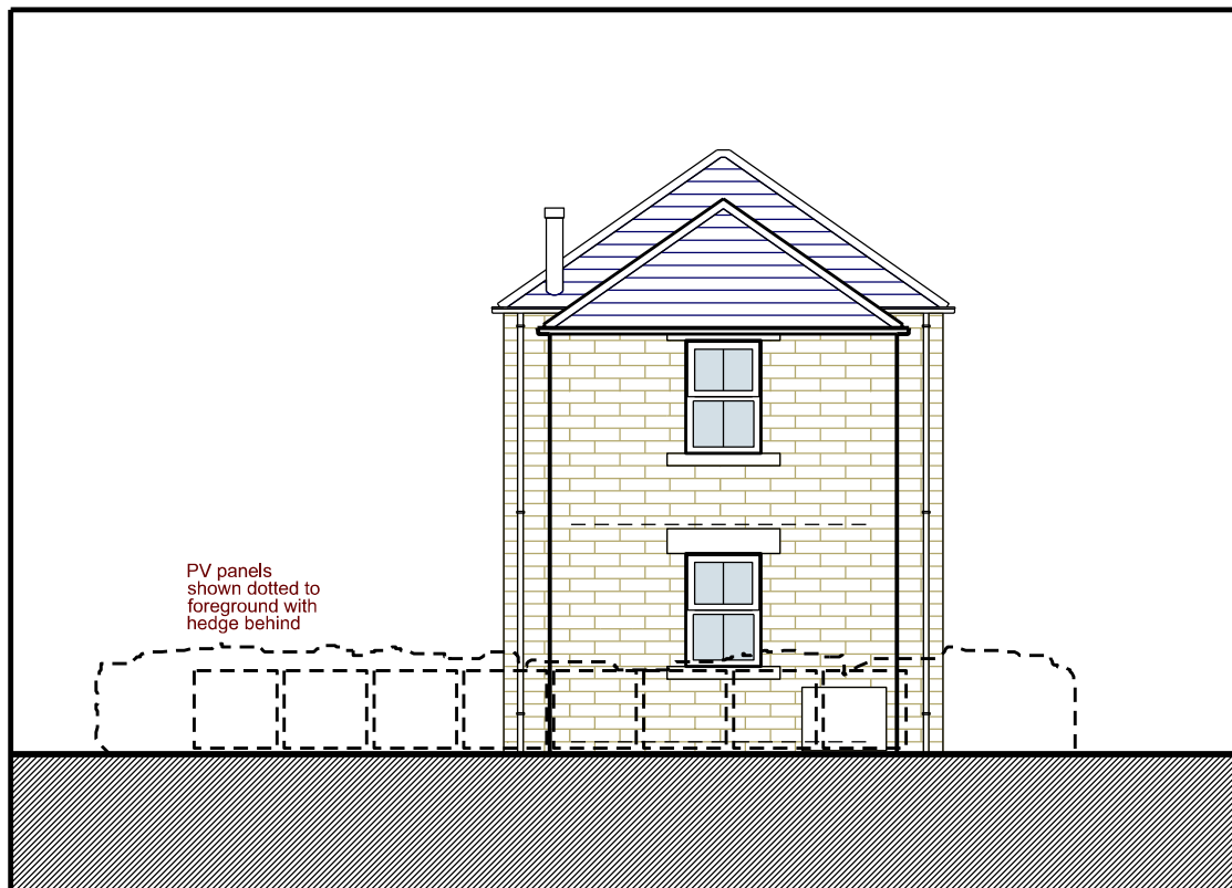
South Elevation - Proposed
