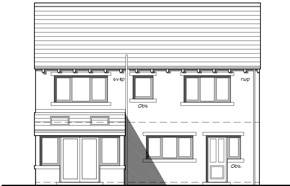
Rear Elevation
