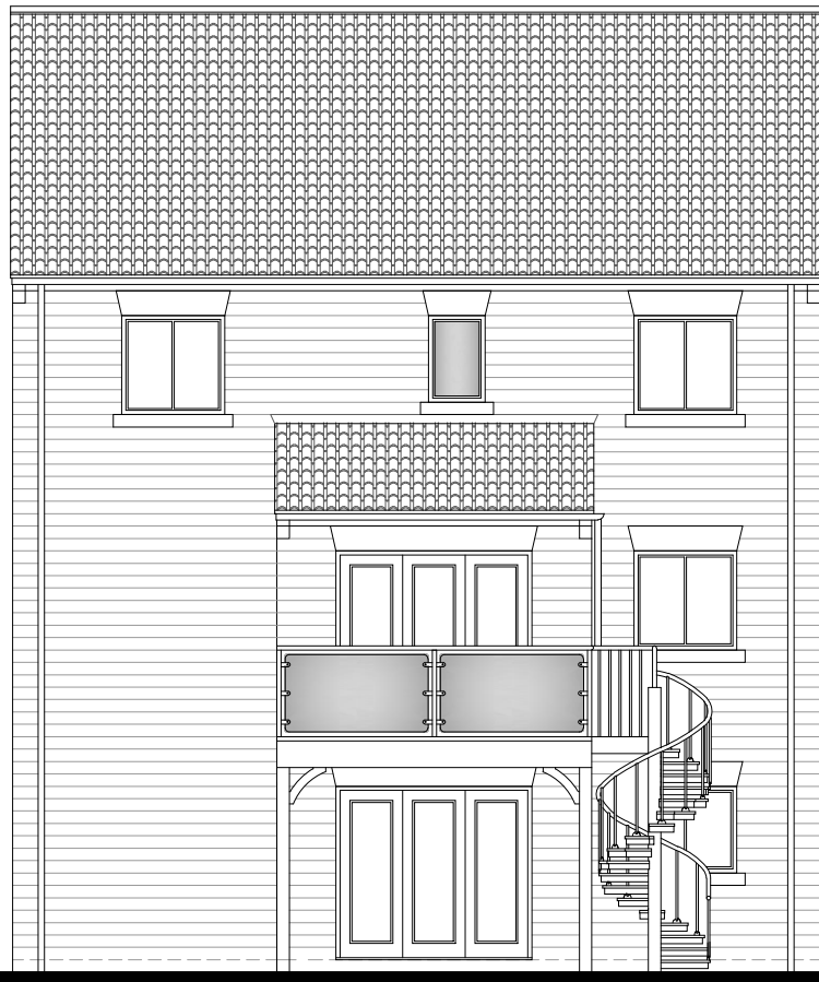
REAR ELEVATION
