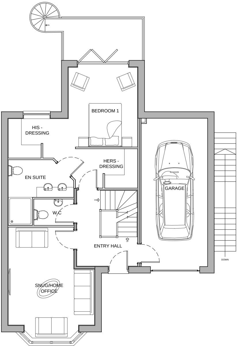
UPPER GROUND FLOOR PLAN
