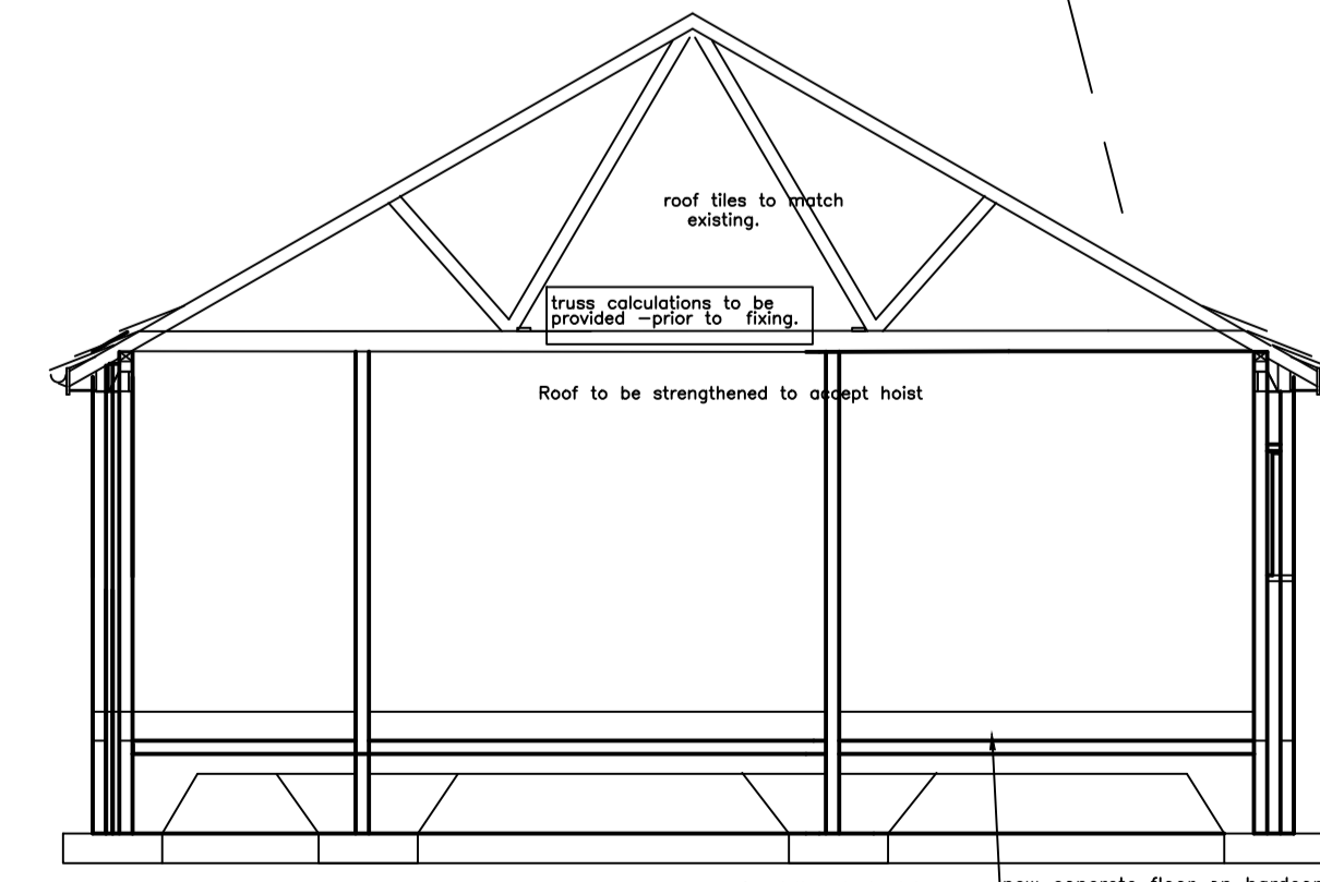
SECTION (typical)
