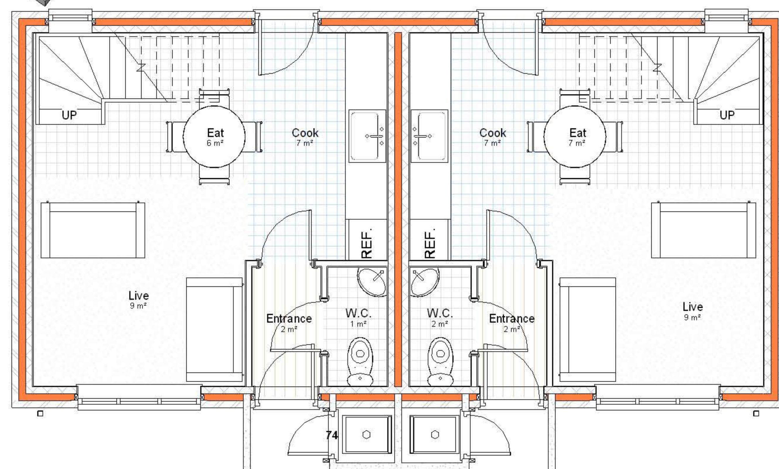
Ground Floor 1:50.
