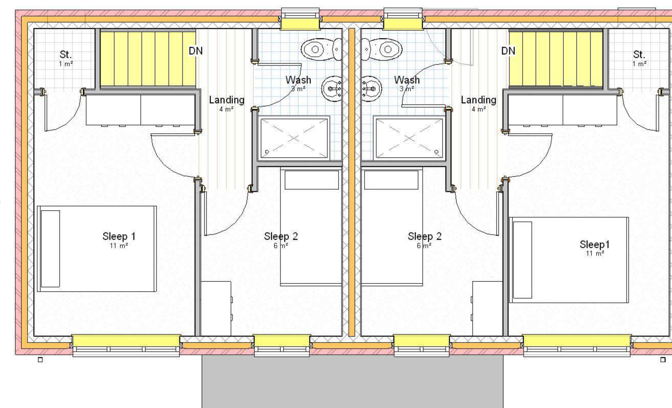
First Floor 1:50.
