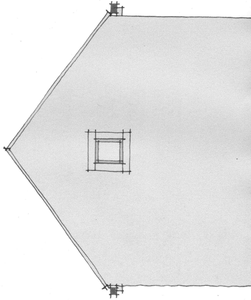
NORTH ELEVATION
