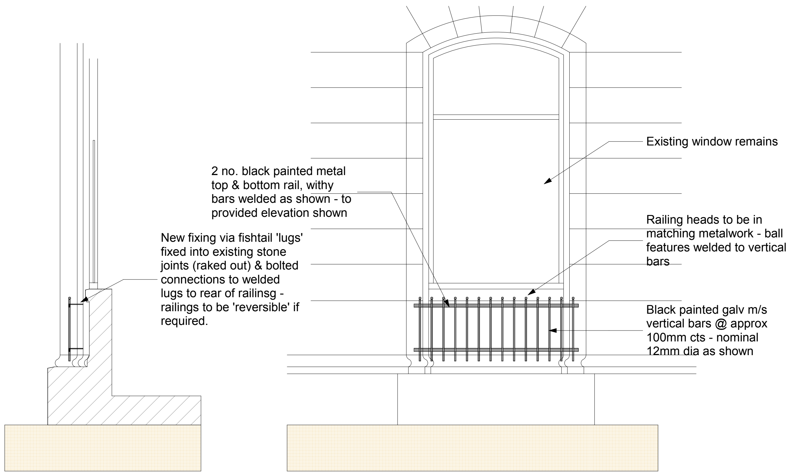
EXPANDED ELEVATION - AS PROPOSED
