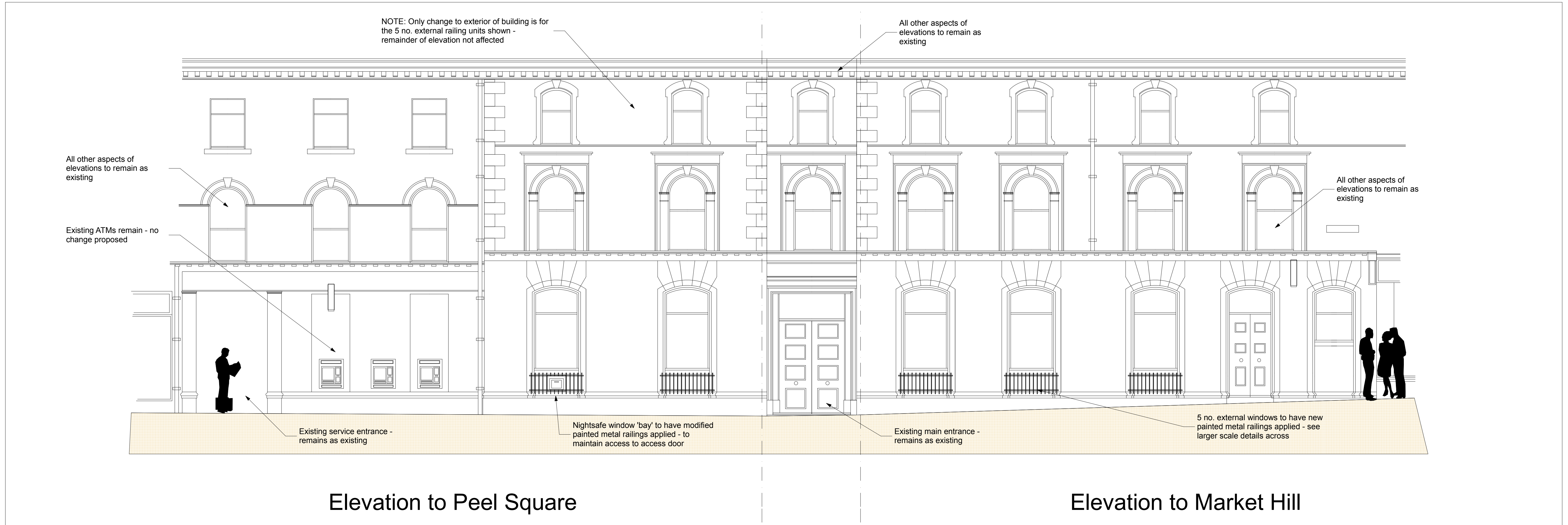
EXPANDED ELEVATION - AS PROPOSED
