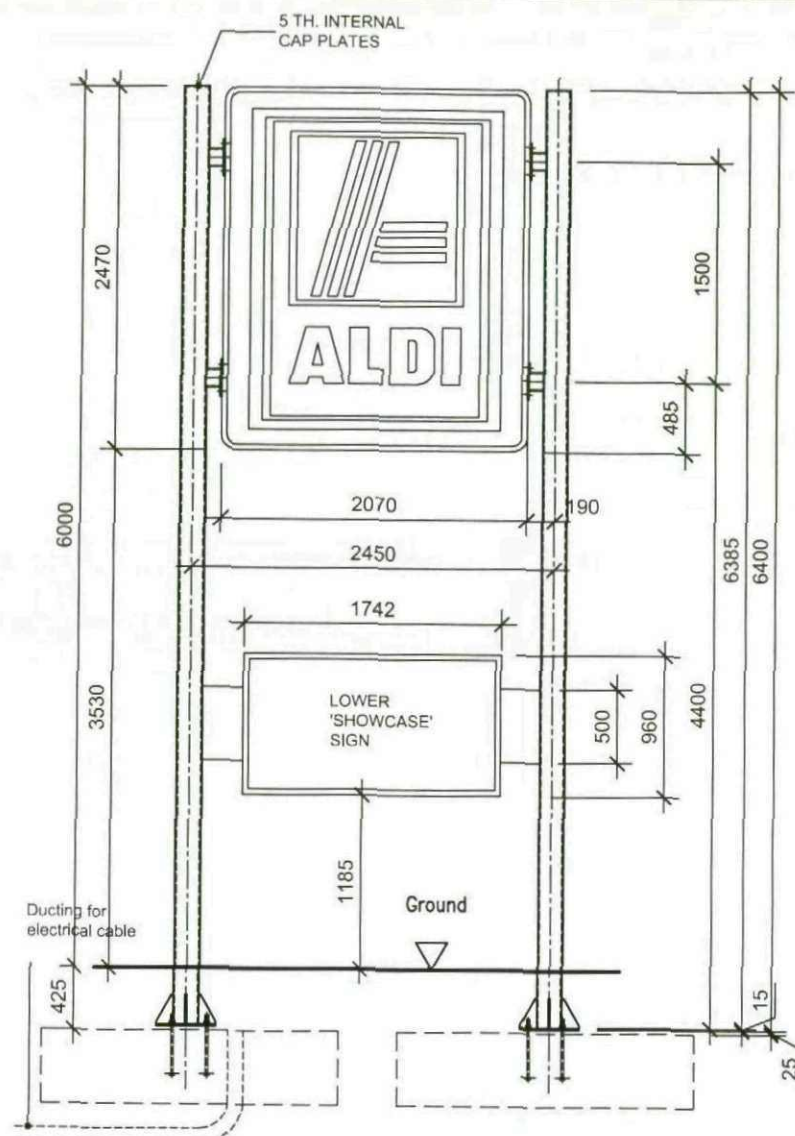
ELEVATION ON STANDARD SITE ENTRANCE SIGN 3.530m GROUND TO U/S OF SIGN
