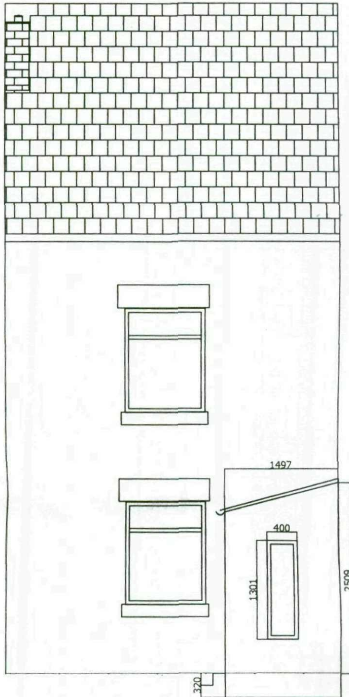
front elevation
