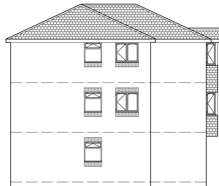
SIDE ELEVATION
