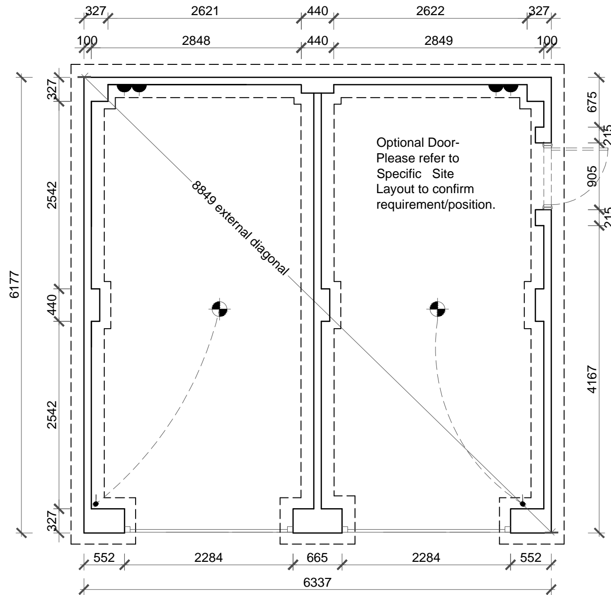
FOUNDATION PLAN
