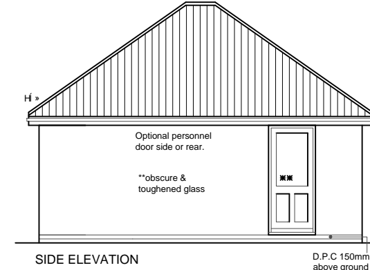
SIDE ELEVATION
