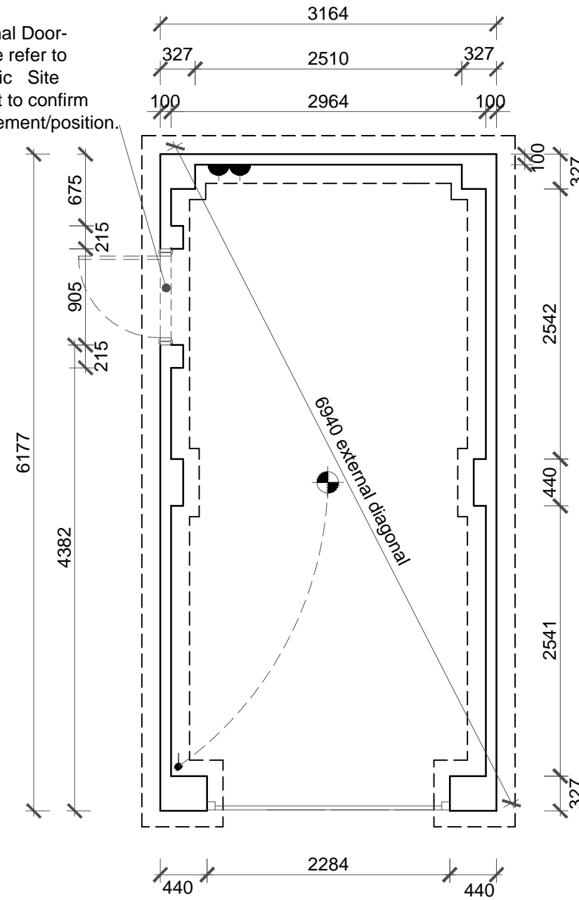
FOUNDATION PLAN
