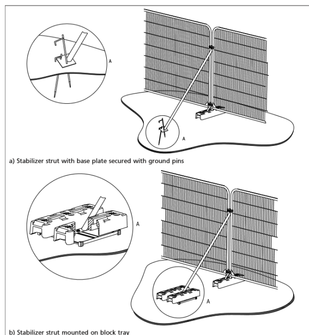
Fig 2: Examples of above ground stabilizing systems BS 5837:2012 –Trees in relation to Design, Demolition and Construction
