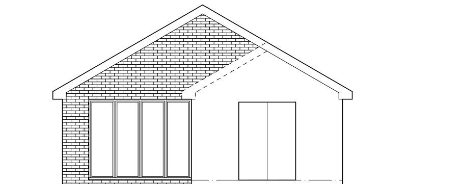
REAR ELEVATION
