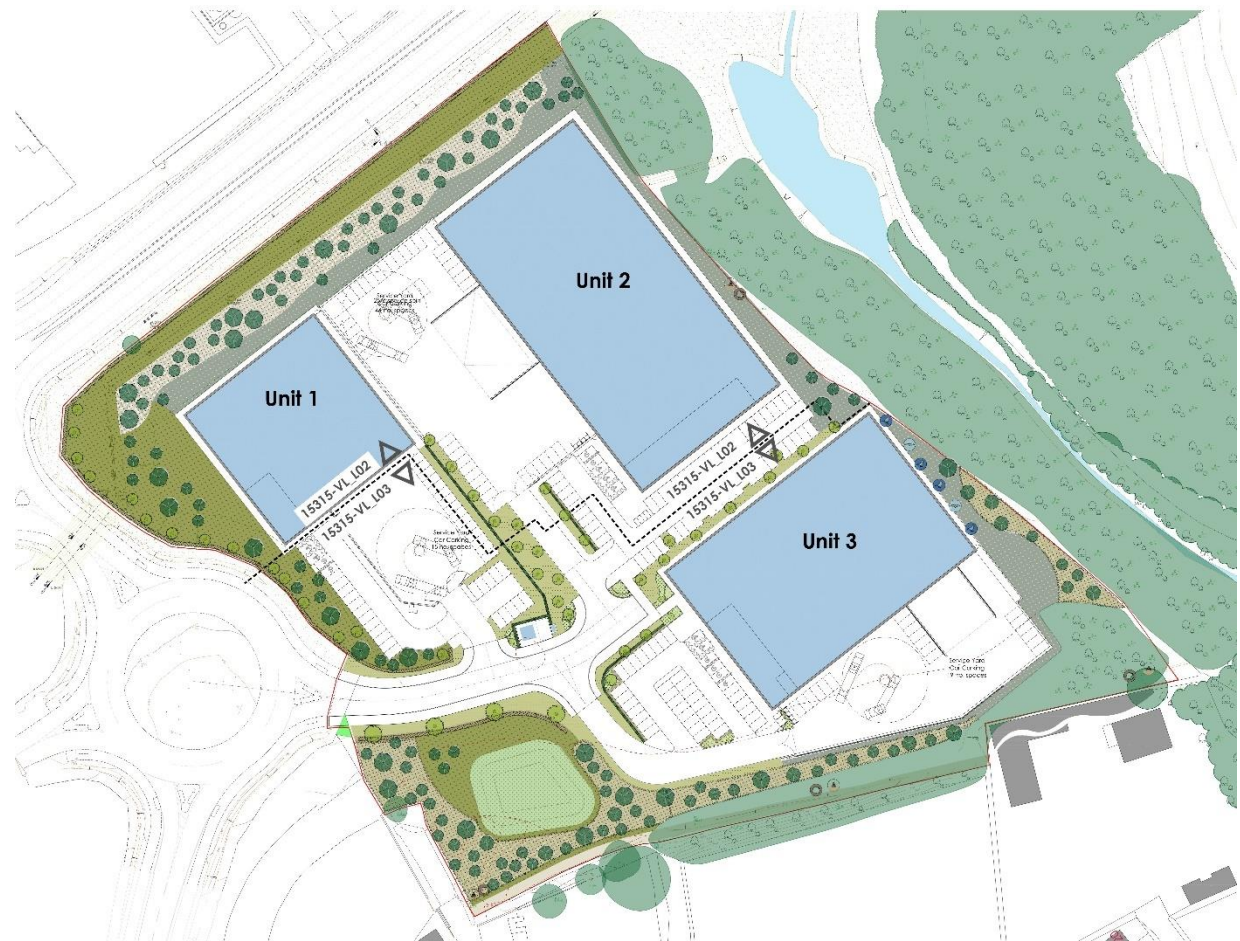
Figure 4.1 Landscape Masterplan (dwg. 15315-VL_L01 rev. H, September 2022, Vector Design Concepts).
