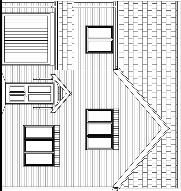
Front Elevation
