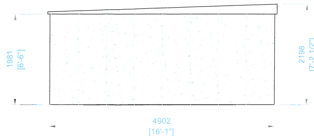
RH ELEVATION
