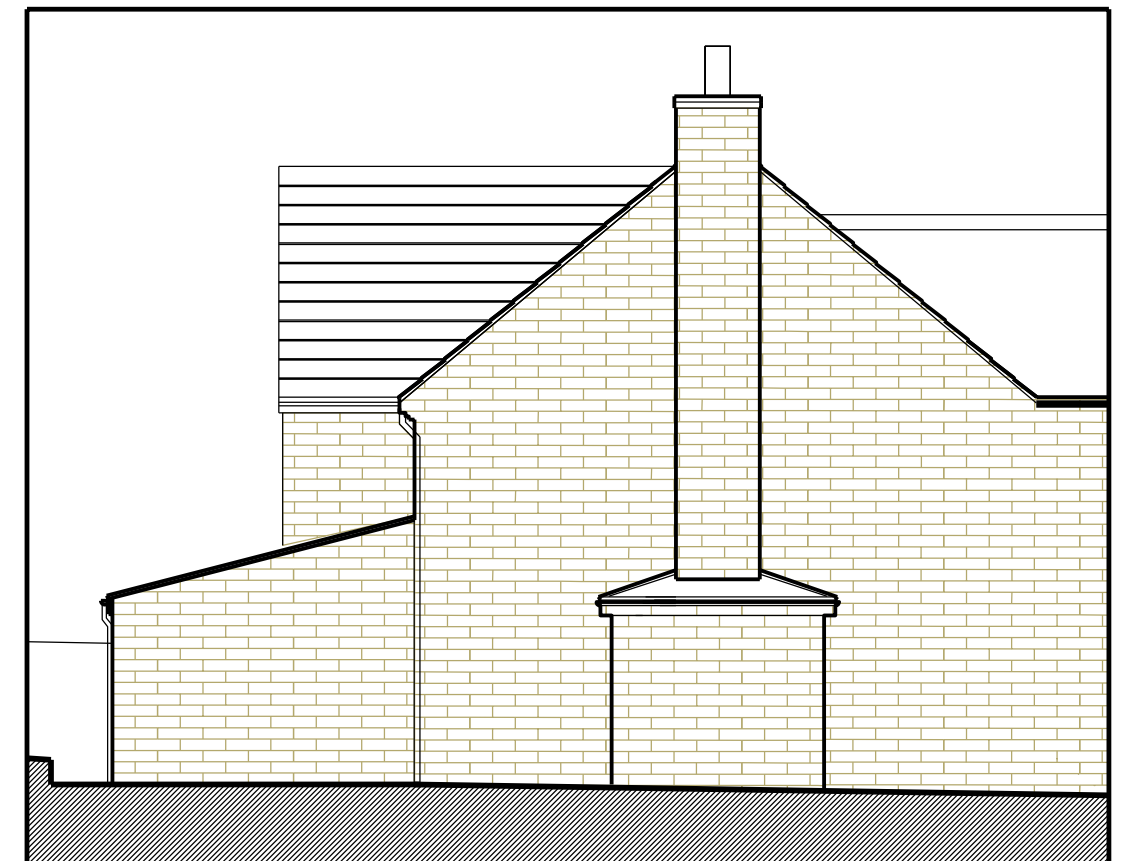
West Elevation - Proposed
