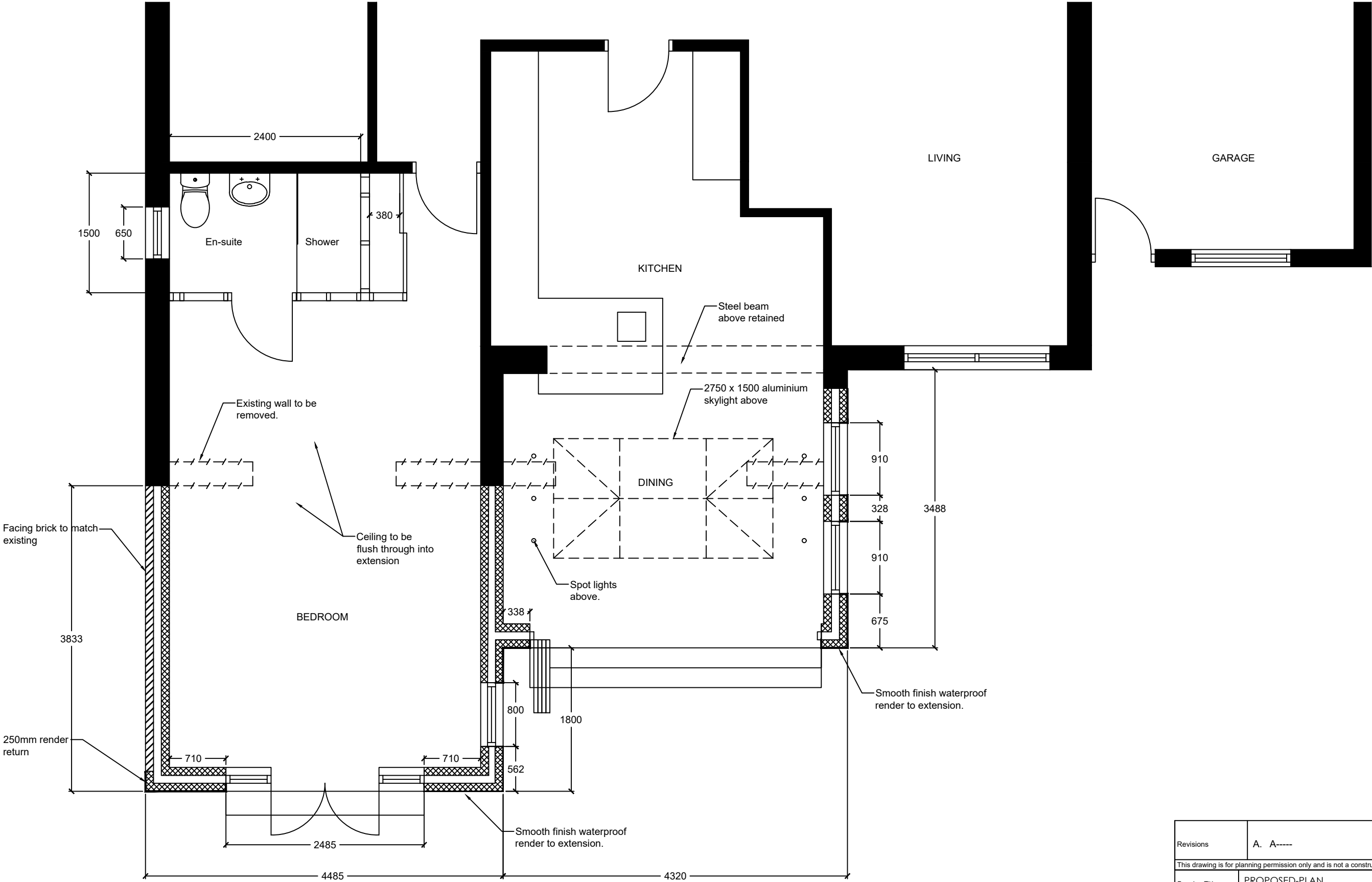
PROPOSED PLAN 1:50
