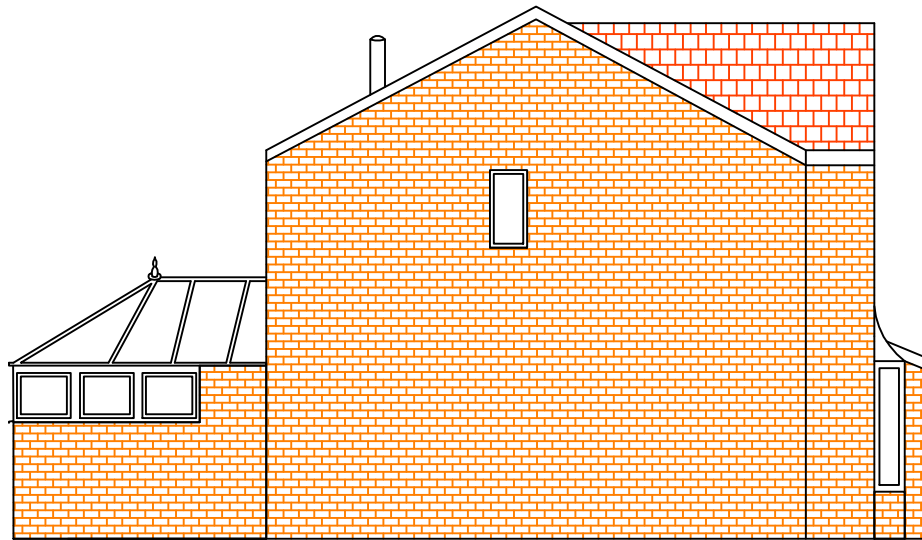
Current Side Elevation
