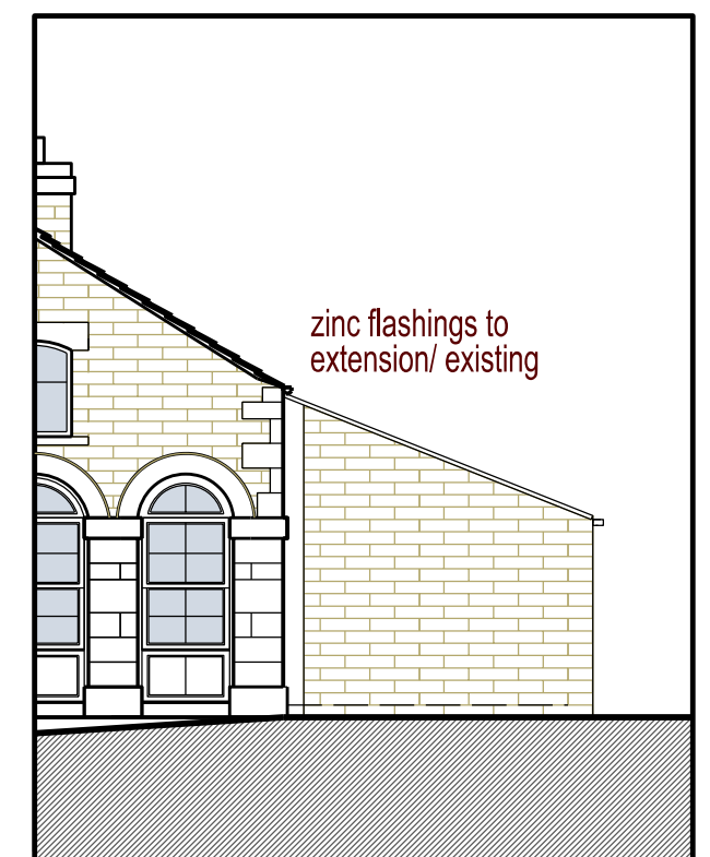
West Elevation - Proposed
