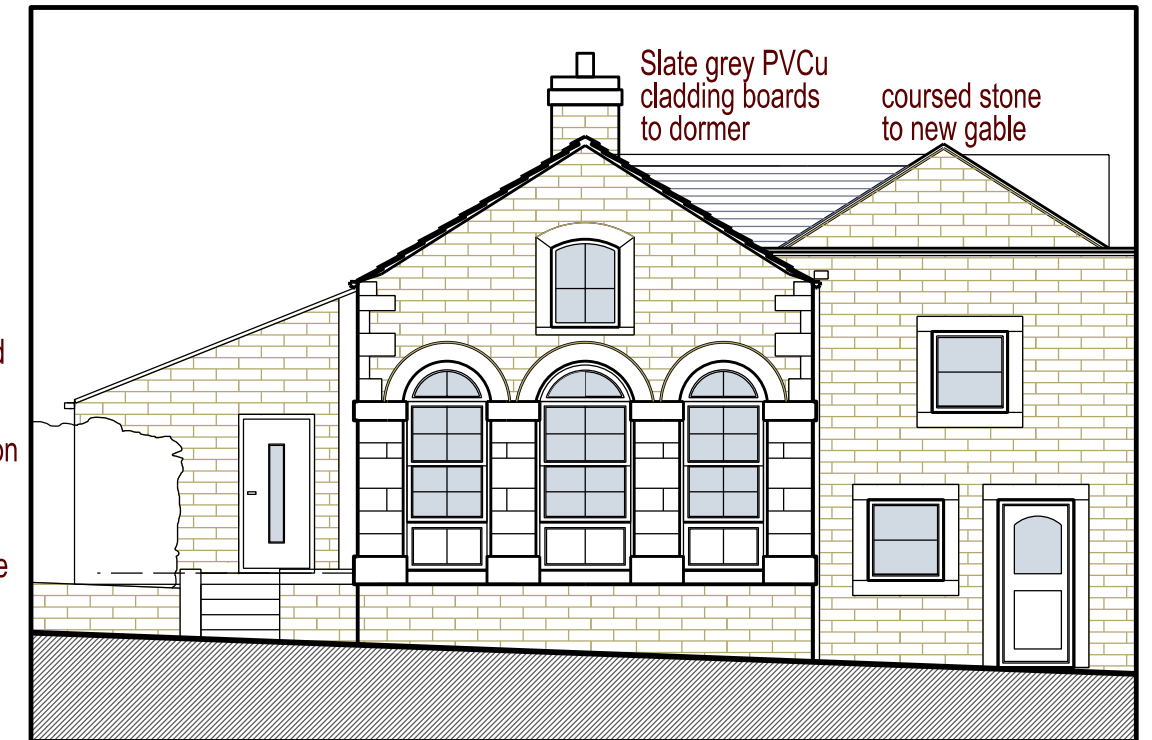
timber framed infill windows to gable East Elevation - Proposed
