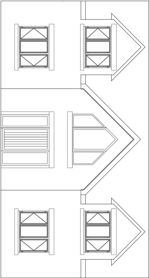
FRONT ELEVATION TO NEWLAND AVENUE
