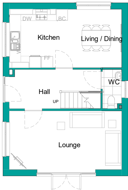
Ground Floor. 1 : 100
