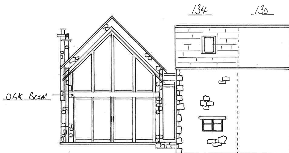
PROPOSED ELEVATION
