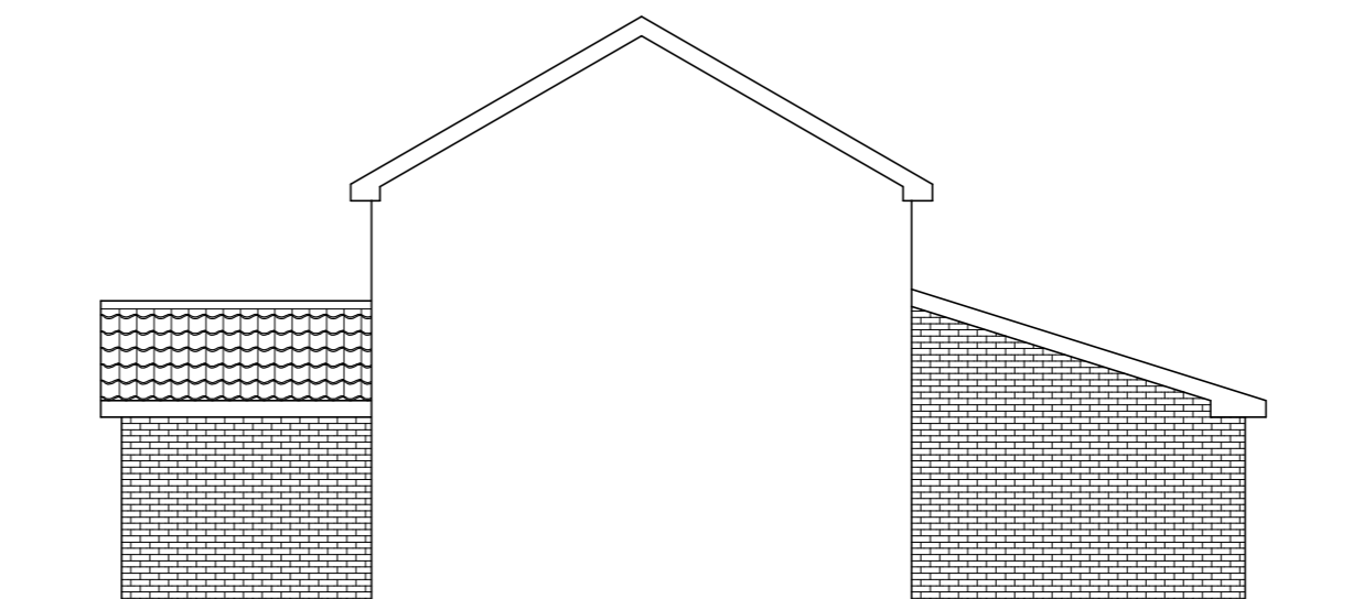
SIDE ELEVATION
