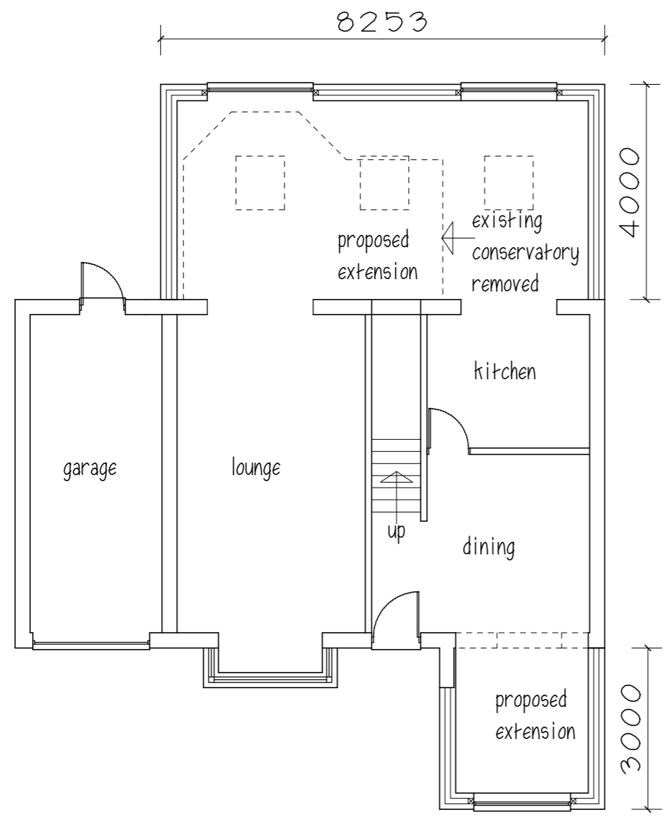
GROUND FLOOR
