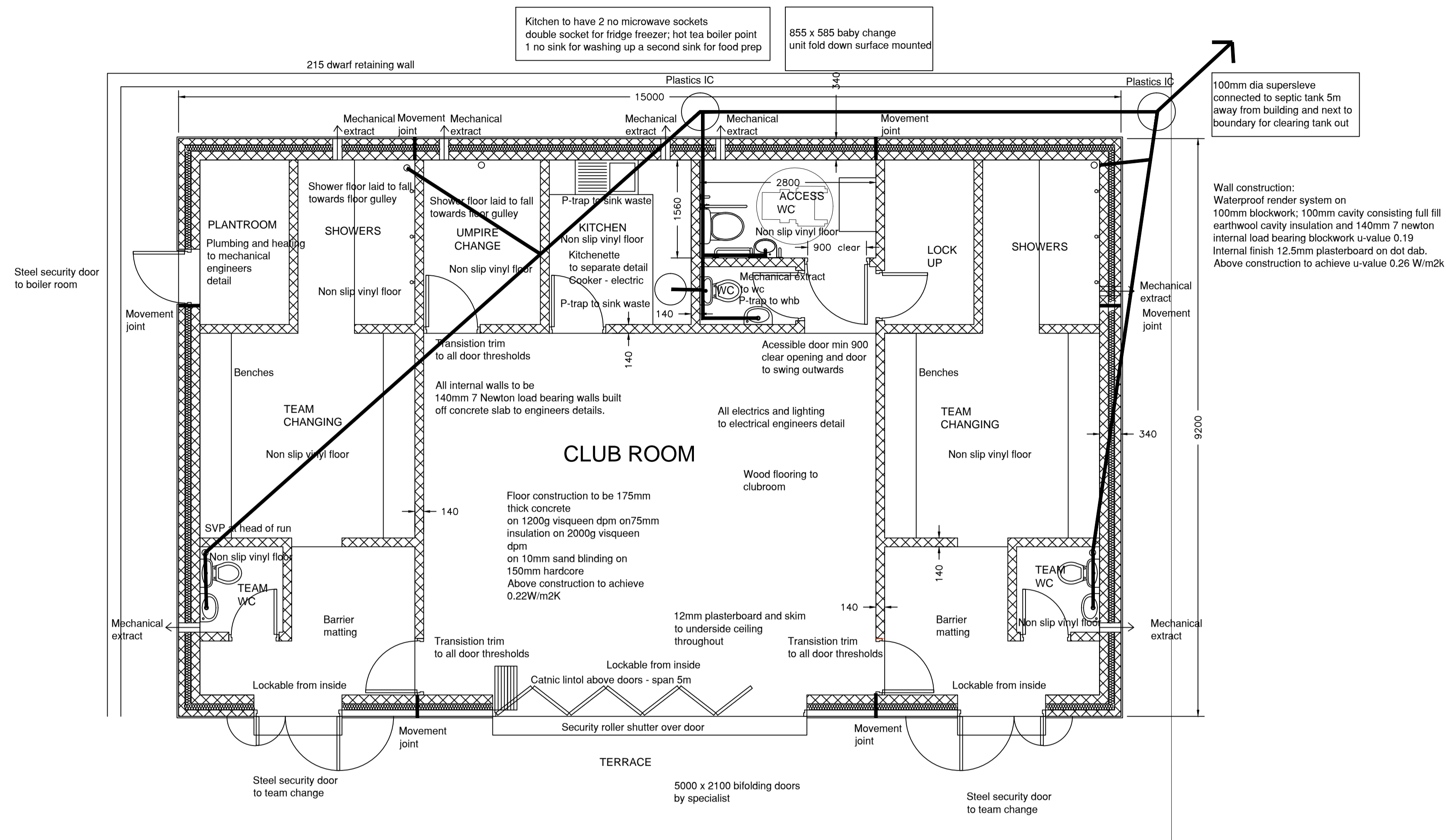
PROPOSED PLAN 1:50
