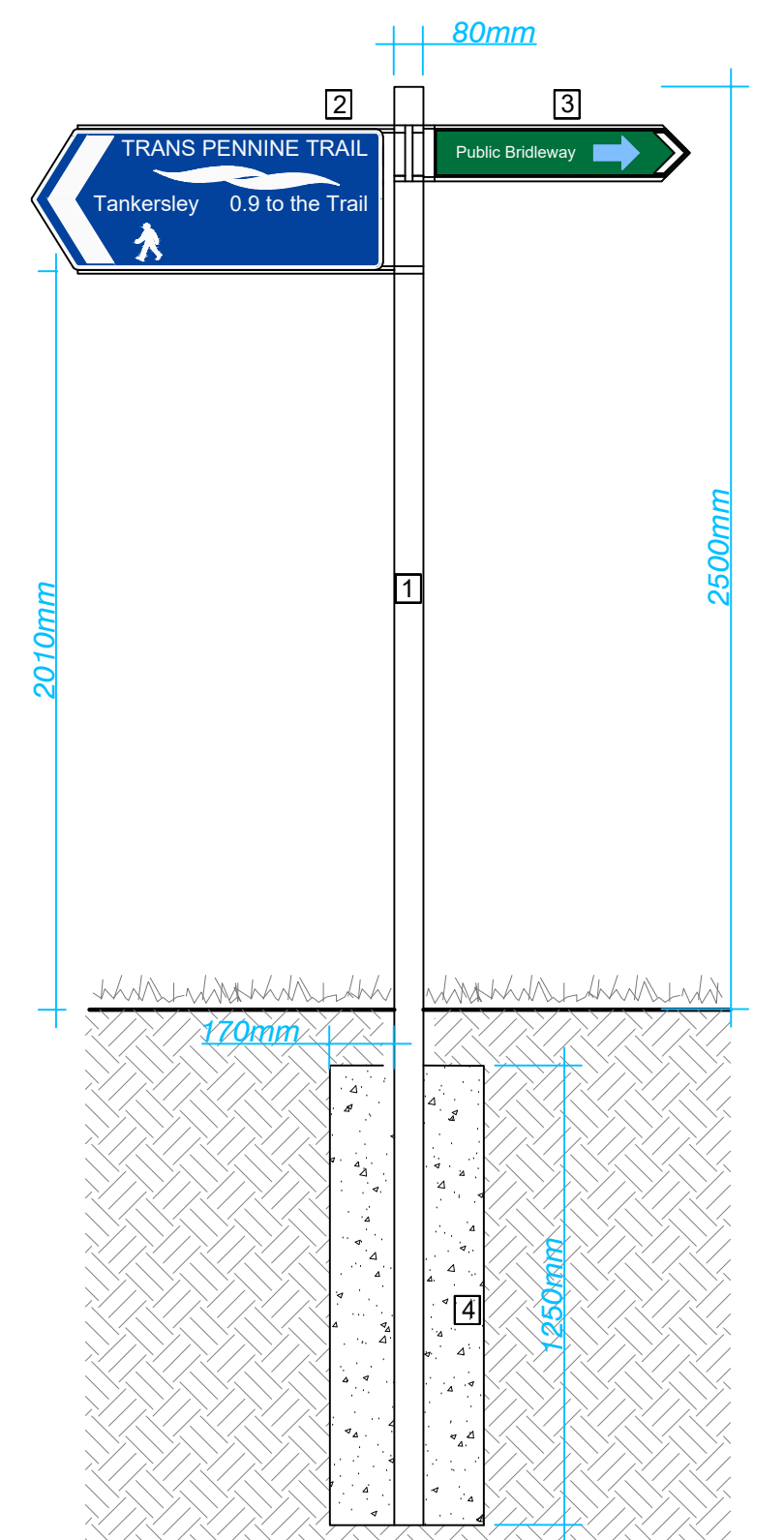
02 TPT Sign 2 - Metal Fingerpost
