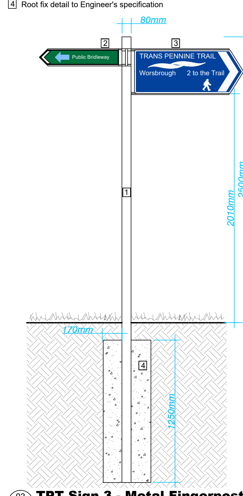
03 TPT Sign 3 - Metal Fingerpost
