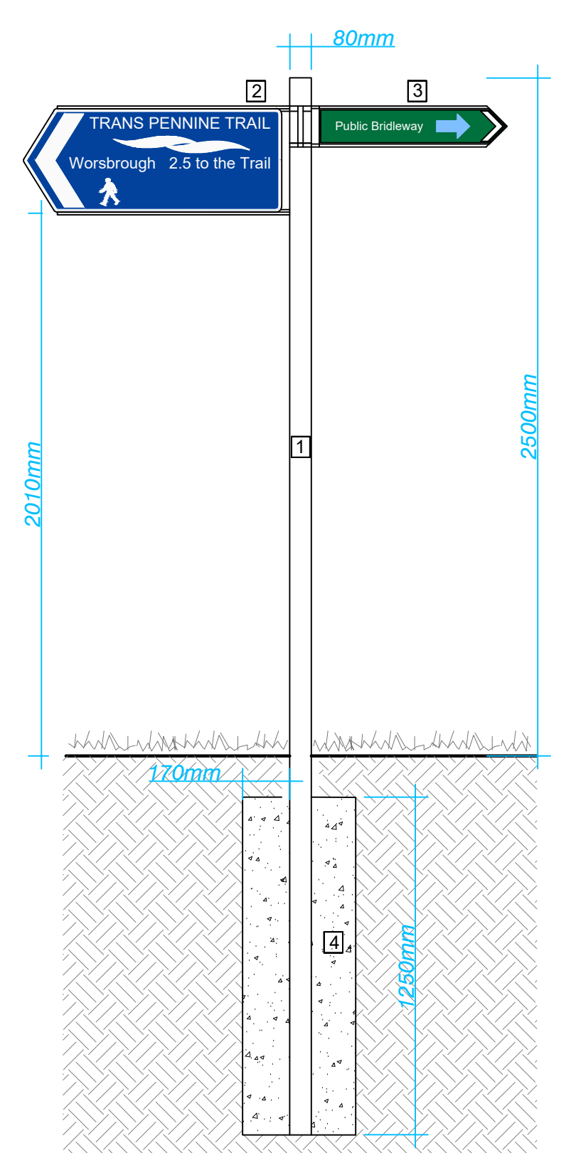
01 TPT Sign 1 - Metal Fingerpost
