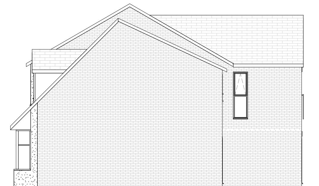
LEFT ELEVATION 1 : 100
