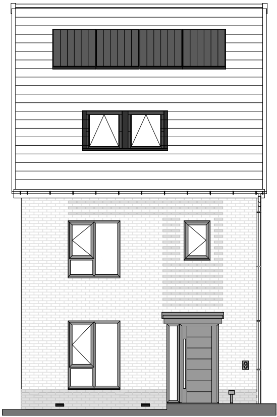
FRONT ELEVATION
