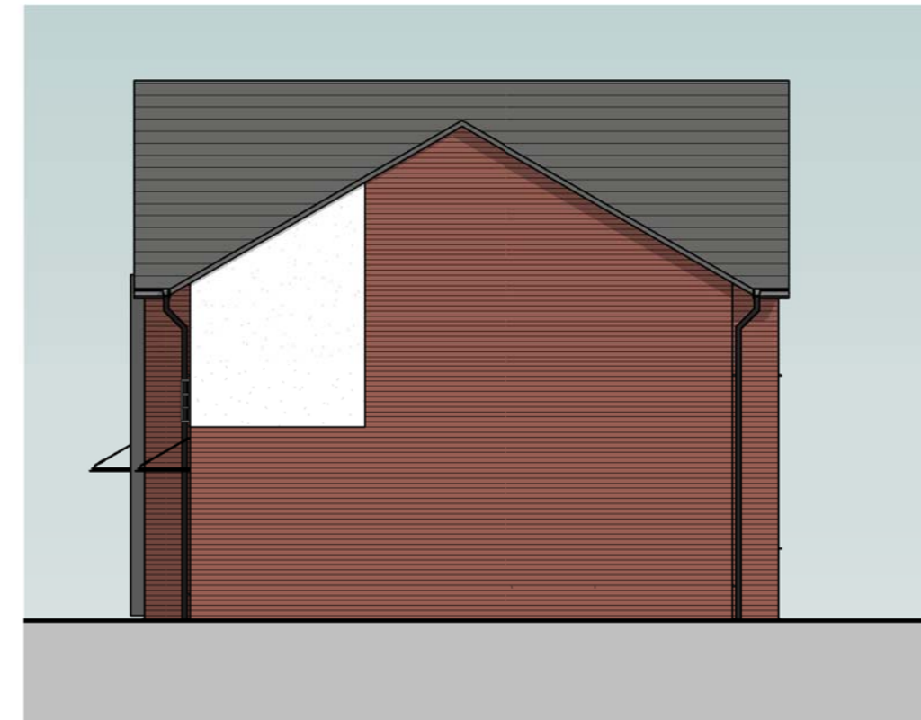
Plot 9 Side / West Elevation 1 : 100
