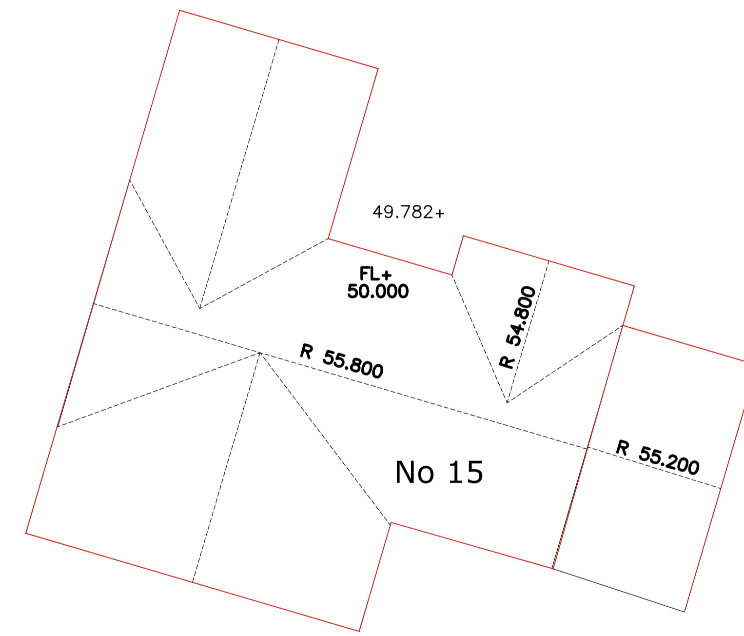
PROPOSED LEVELS SCALE 1:100
