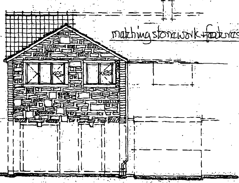
PROPOSED FRONT VIEW.
