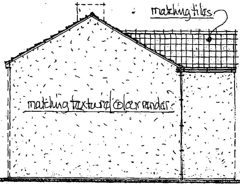
PROPOSED SIDE VIEW FROM NO 54.
