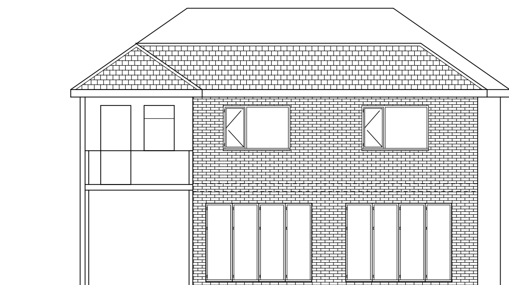
REAR ELEVATION
