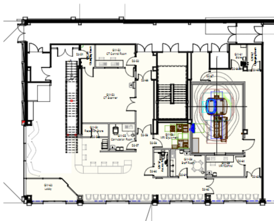
Ground Floor Proposed Plan
