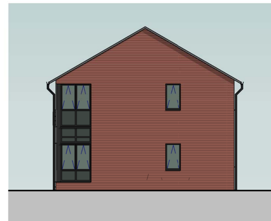
Plot 27 Side / East Elevation 1 : 100
