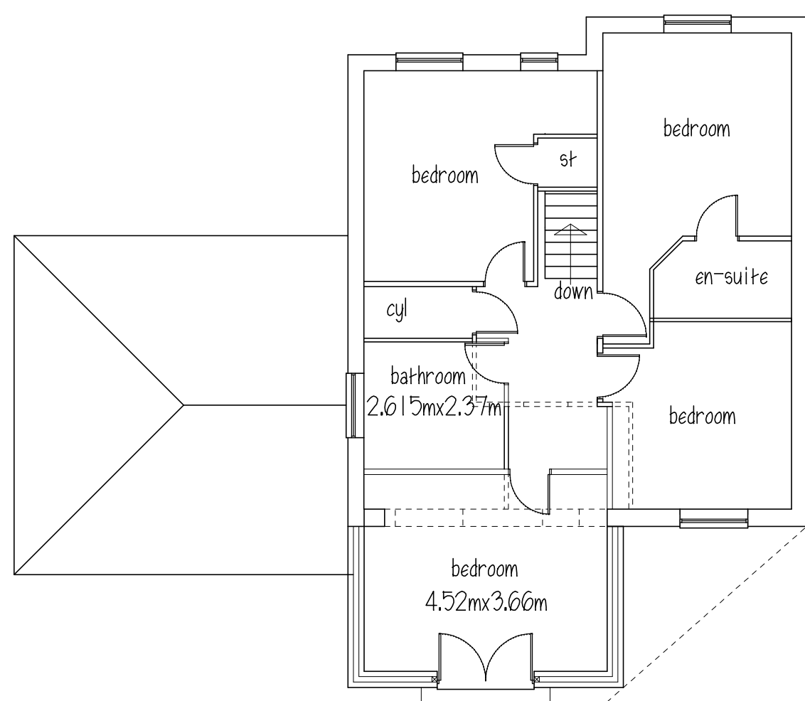
FIRST FLOOR
