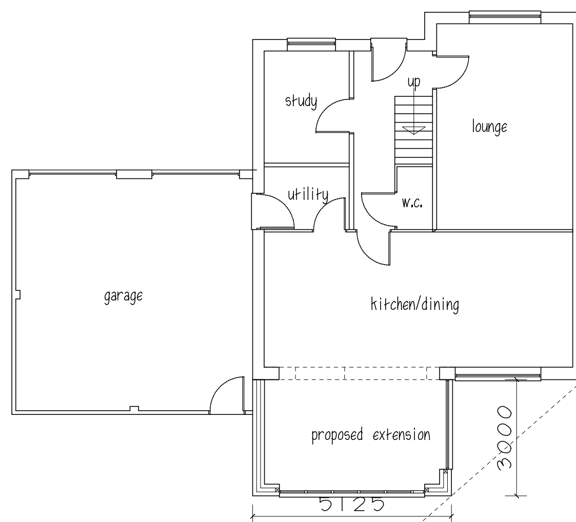
GROUND FLOOR
