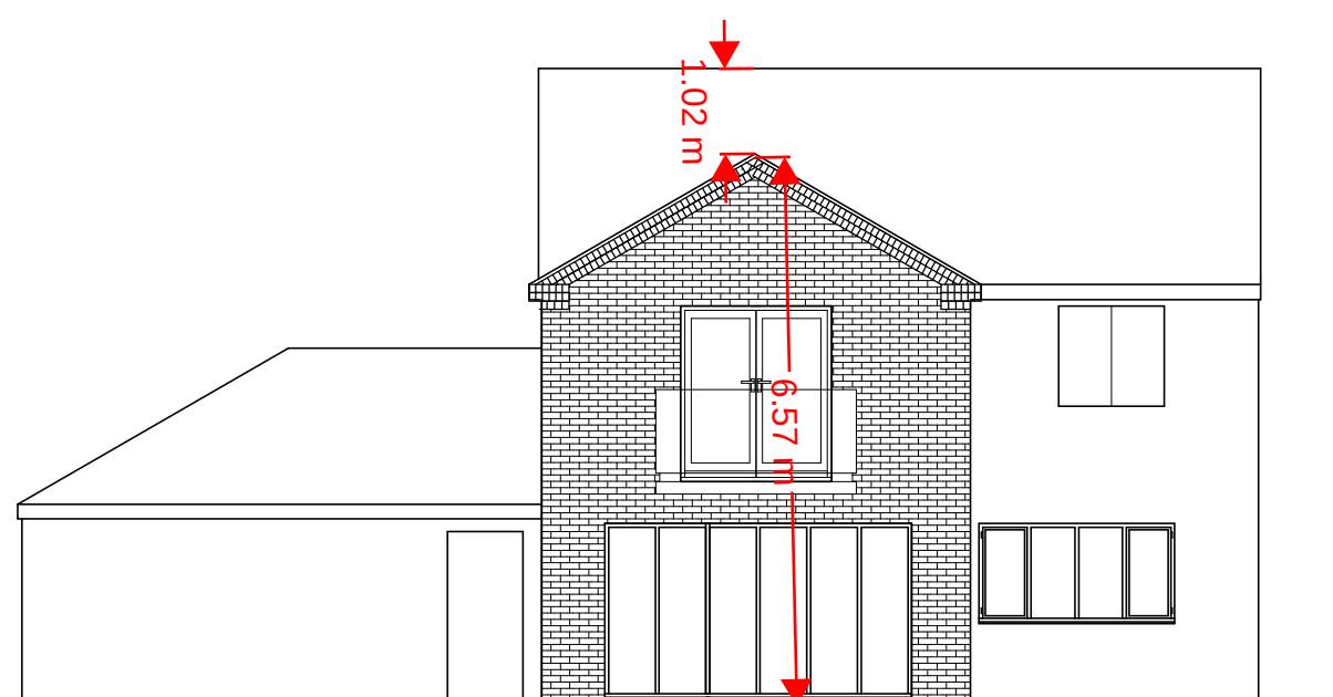
REAR ELEVATION
