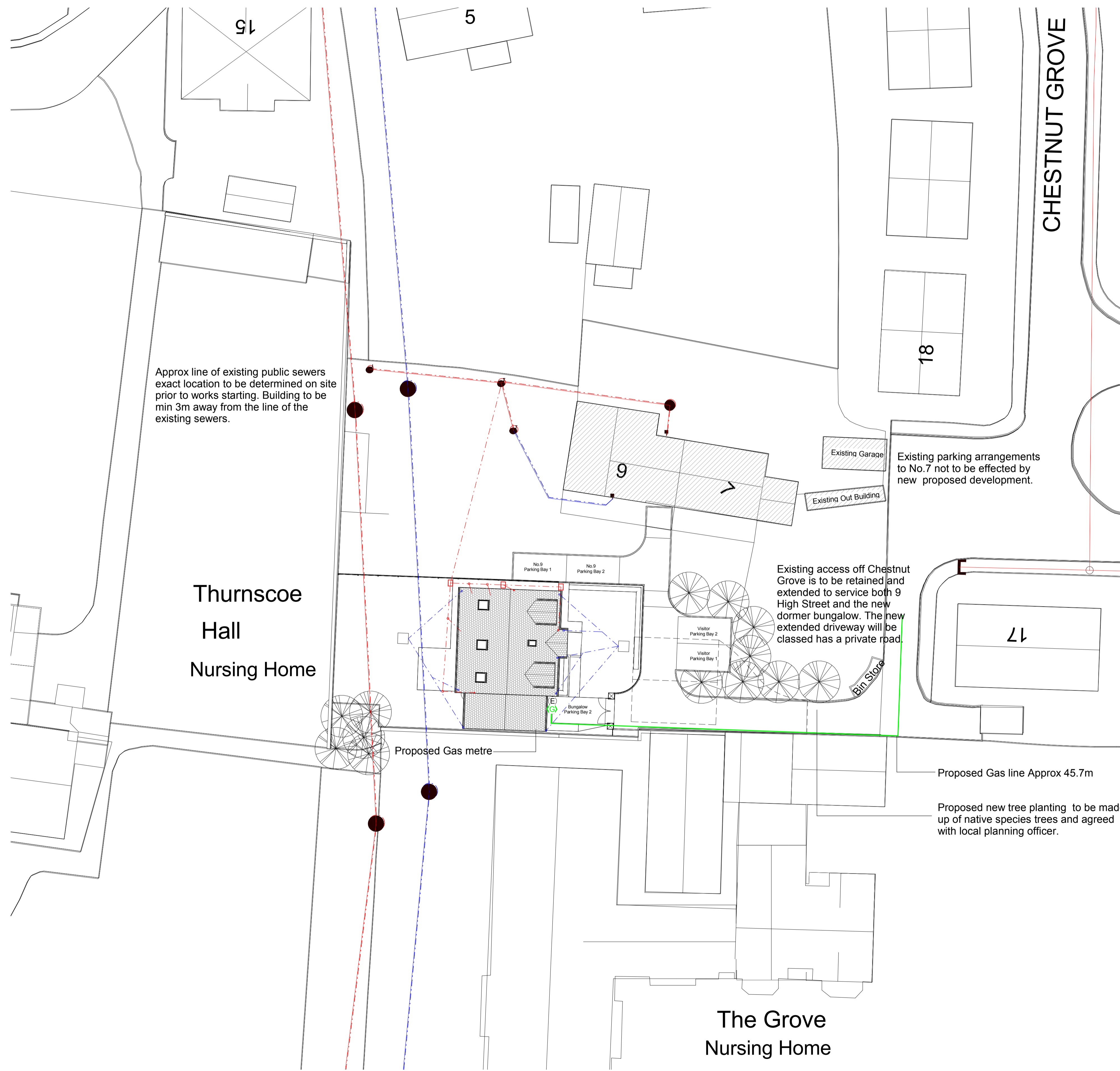
2 Site - Proposed - Site Working Plan 1 : 200
