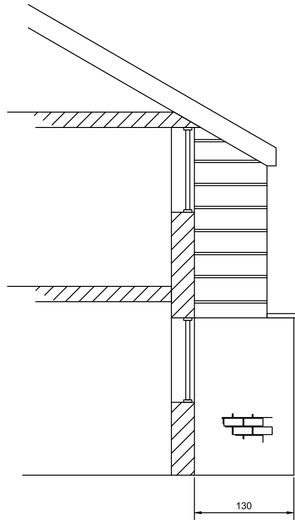
C-C Existing Side Elevation
