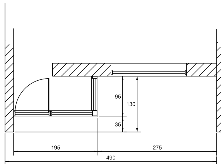
1-1 Existing Floor Plan
