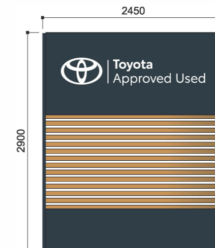
F Double-sided Small Exterior Screen - Toyota Approved Used | 1:50 @ A3
