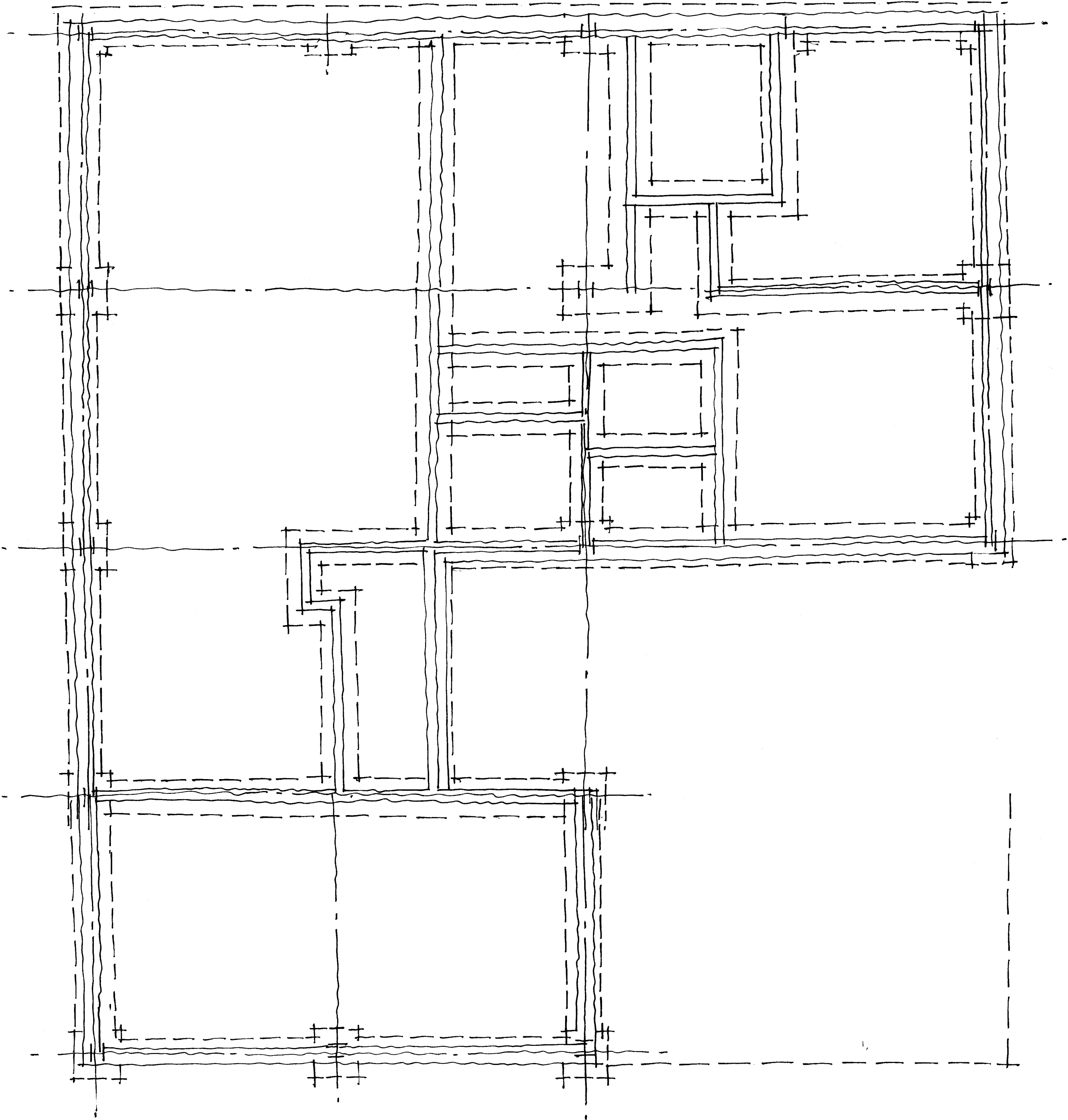
SUBSTRUCTURE PLAN - 1:50
