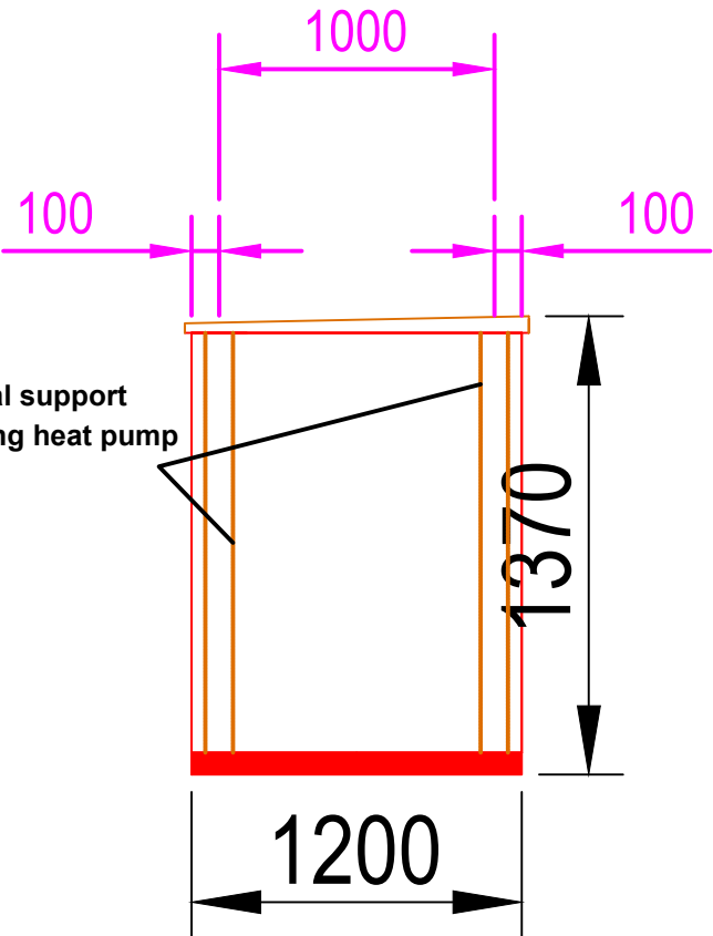
EXTERNAL ELEVATION WALL 2 (SIDE WALL)
