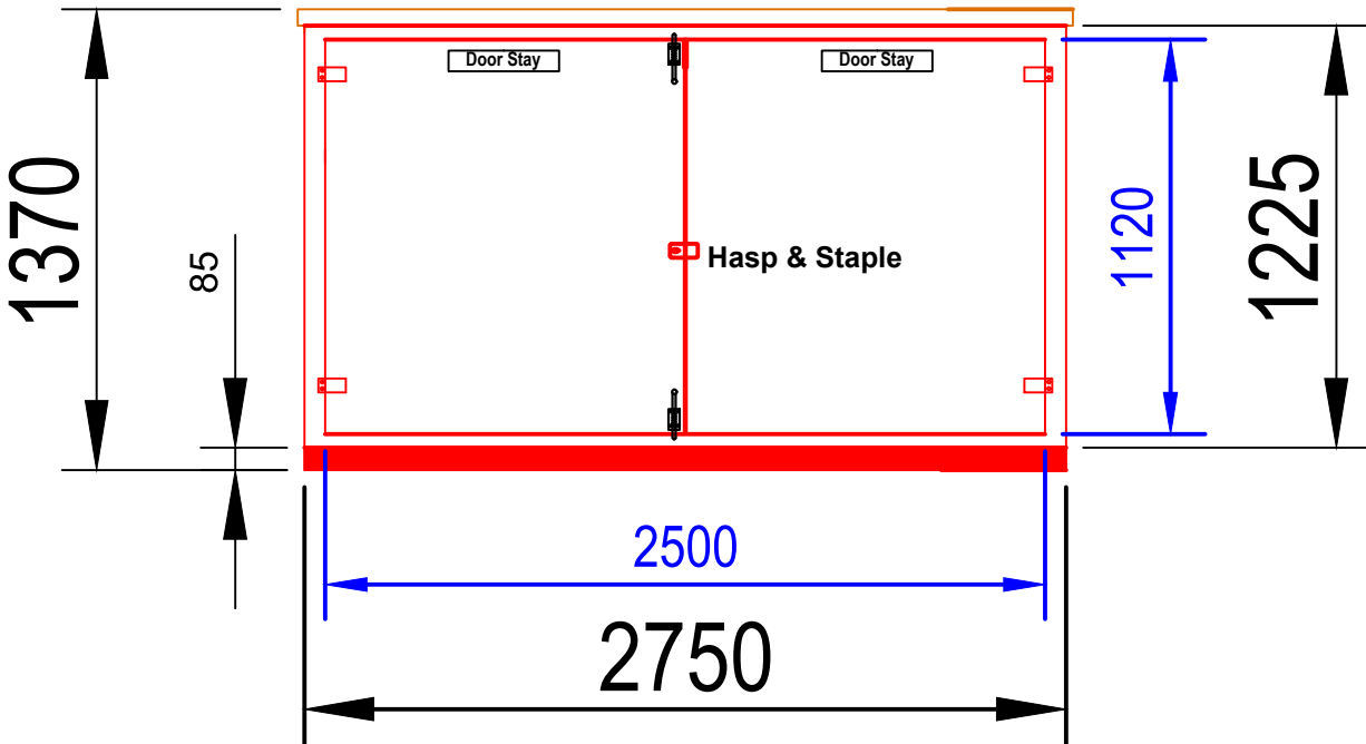
EXTERNAL ELEVATION WALL 1 (FRONT WALL)
