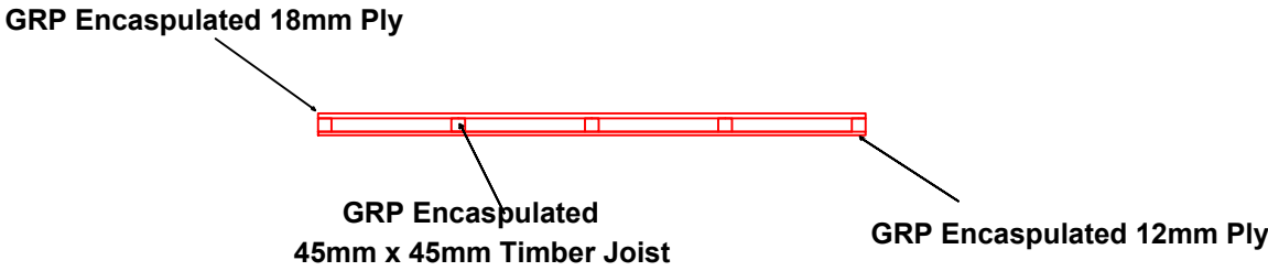
CROSS SECTION OF LOAD BEARING FLOOR
