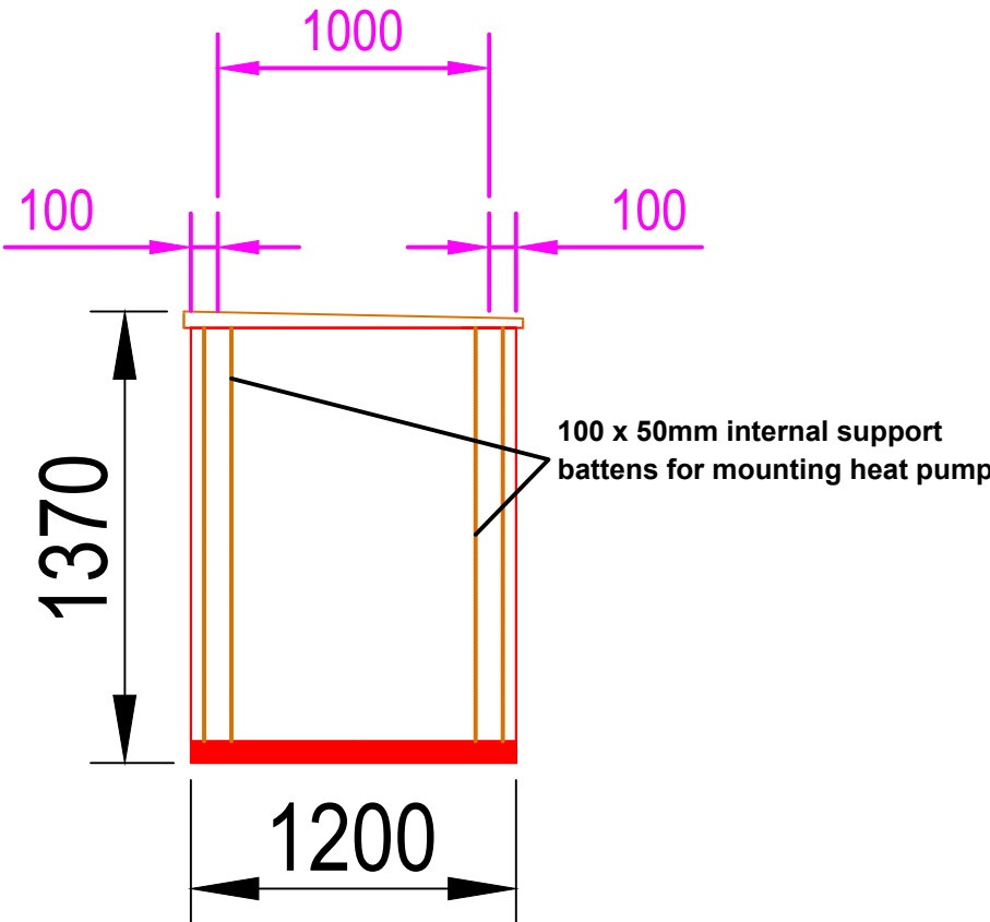
EXTERNAL ELEVATION WALL 4 (SIDE WALL)
