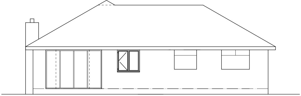
REAR ELEVATION
