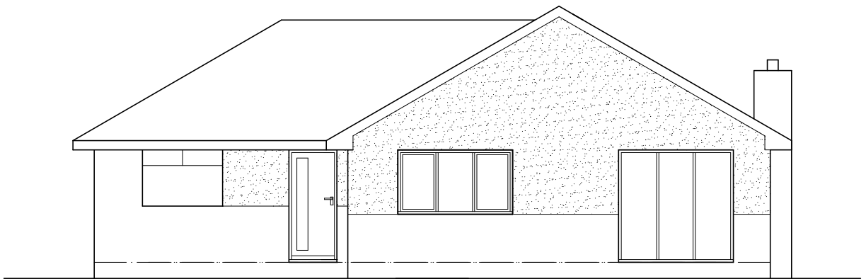
FRONT ELEVATION
