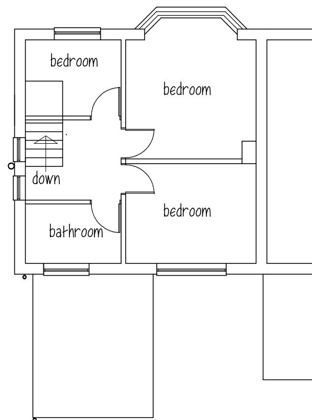
EX FIRST FLOOR
