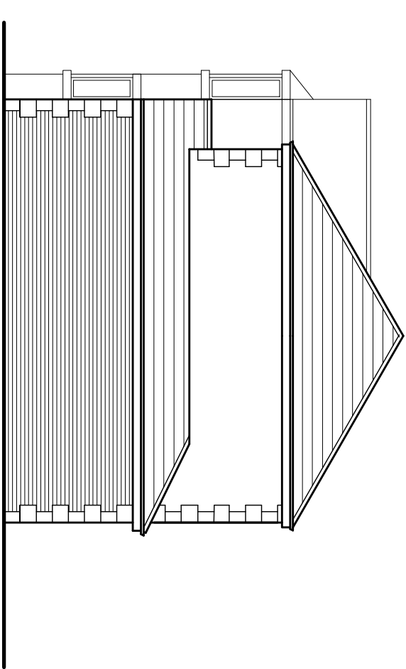
side elevation -as proposed
