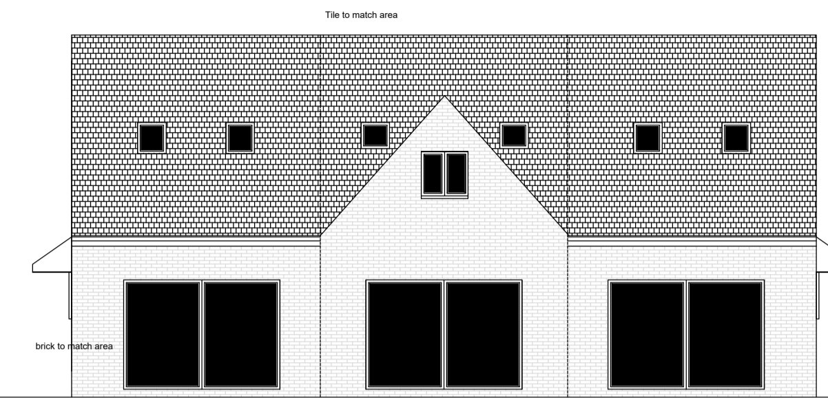
Rear Elevation 1:100
