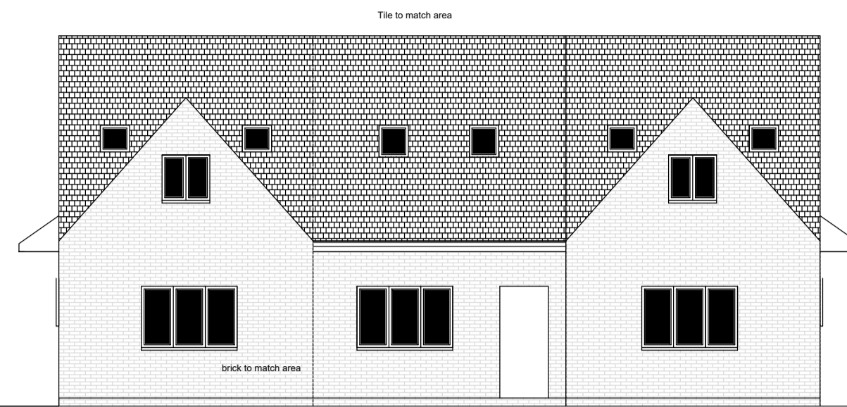
Front Elevation 1:100
