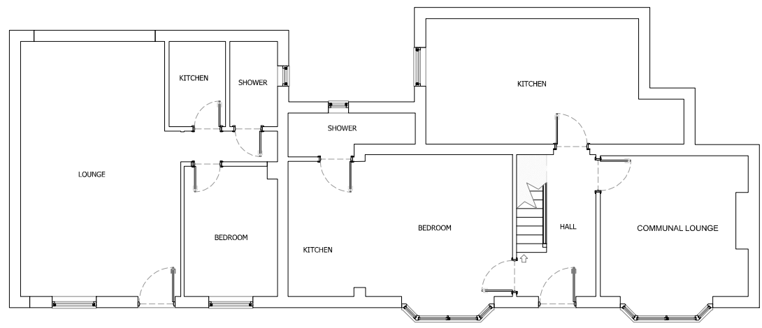
PROPOSED GROUND FLOOR 0 1 2 3 4 5 1:50
