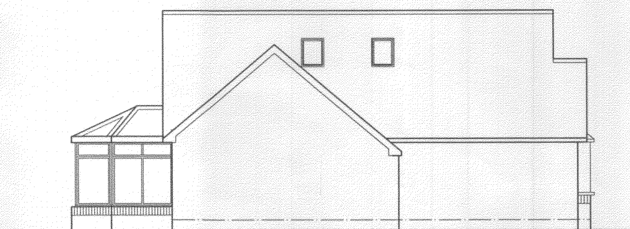
SIDE ELEVATION
