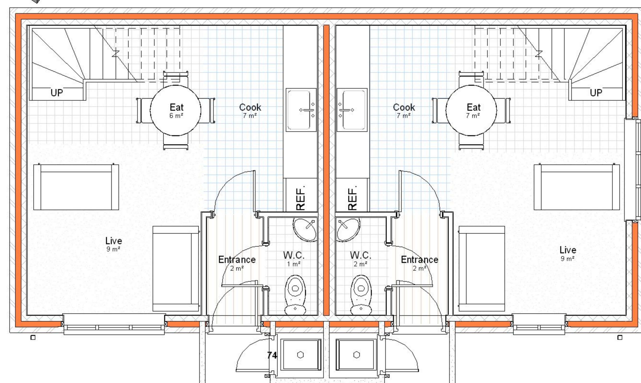
Ground Floor 1:50.
