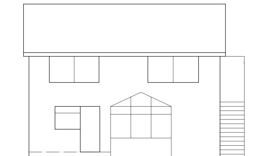
REAR ELEVATION
