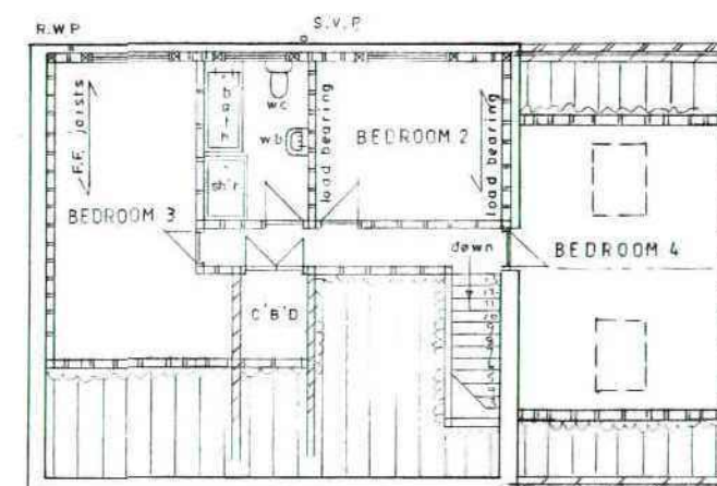
PROPOSED F.F. PLAN
