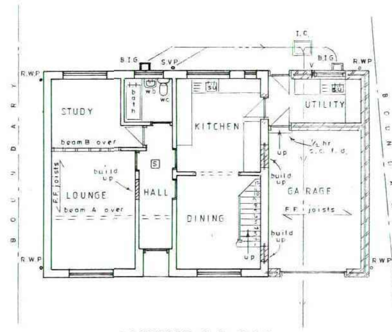
PROPOSED G.F. PLAN
