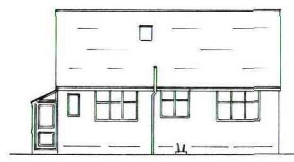
EXISTING REAR EAST
